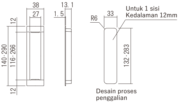
Lapisan Chrome (Panjang : 290) Hairline Cat Putih Cst Hitam
